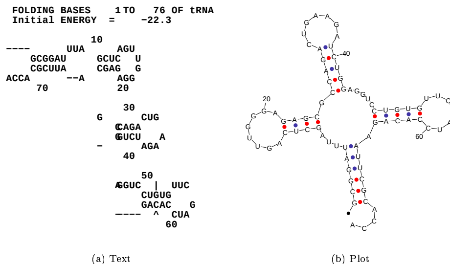
Figure 11: The second and final folding of S. cerevisiae Phe-tRNA at 37°, with P=5% and W=3 (default values). (a) The selected base pair is G 51 -C 63 . The base numbers are placed so that the least significant digit, always a 0, is above or below the enumerated base. (b) The usual plotted representation. The efn2 program has adjusted \Delta G from -22.3 to -22.7 kcal/mole
