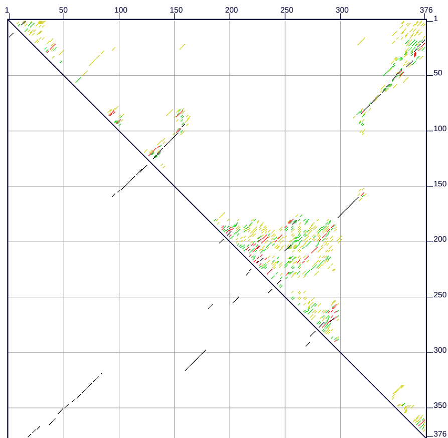
Figure 17: The energy dot plot for the “Example 3” sequence, with \Delta G = -196.3 kcal/mole and \Delta\Delta G = 9.8 kcal/mole. The region from bases 180 to 295 shows a great deal of uncertainty in its folding. This may be interpreted as a large ensemble of different foldings, or simply an “unstructured” region. In contrast, the long stem pairing bases 160-178 with 316-298, respectively, is extremely well determined. Also well-determined is a stem loop region that stretches from 37-81 and 322-365.
